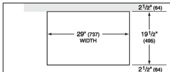
COUNTERTOP CUT-OUT
